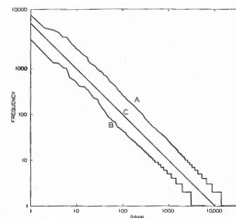
Fig. 2-1. The rank-frequency distribution of words. (A) The James Joyce data; (B) the Elledge data; (C) ideal curve with slope of negative unity.
