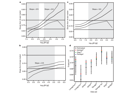
Figure 2 | Scaling exponent depends on mass range. a, Slopes estimated by linear regression within a three log-unit mass range (smaller near the boundaries). Values on the abscissa denote mass log 10 within the range. When the 95% confidence regions (dashed lines) include the 2/3 or 3/4 lines, the local slope is consistent with a 2/3 or 3/4 exponent, respectively. These cases are indicated by the shaded regions (2/3 on the left and 3/4 on the right). b, Slopes estimated by using all data points with 30 < c. The shaded region is consistent with 2/3 slope estimates. d, Slopes estimated by using all data points with 30 < c. The shaded region is consistent with 3/4 slope
