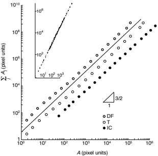
Figure 2 Allometric scaling in river networks. Double logarithmic plot of C = \sum A_i A_j versus A for three river networks characterized by different climates, geology and geographic locations (Dry Fork, West Virginia, 586 km 2 , digital terrain map (DTM) size 30 × 30 m 2 ; Island Creek, Idaho, 280 km 2 , DTM size 30 × 30 m 2 ; Tirso, Italy, 2,024 km 2 , DTM size 237 × 237 m 2 ). The experimental points are obtained by binning total contributing areas, and computing the ensemble average of the sum of the inner areas for each sub-basin within the binned interval. The figure uses pixel units in which the smallest area element is assigned a unit value. Also plotted is the predicted scaling relationship with slope 3/2. The inset shows the raw data from the Tirso basin before any binning
