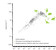
Figure 4 | Predicting the maximum speed of active species with the time-dependent model. The model predictor (grey line) is fitted to data of extant species (grey circles) and extended to higher body masses. Speed data for dinosaurs (green triangles) came from detailed morphological model calculations (values in Table 1) and were not used to obtain model parameters.
