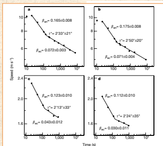
Figure 1 Plots of world record mean speeds against the record time (at November 1999). a,b , Running, and c,d , swimming records: for men ( a,b ), we consider 11 races (200 m, 400 m, 800 m, 1,600 m, 1,500 m, the mile, 3,000 m, 5,000 m, 10,000 m, 1 hour, and marathon); the same races are considered for women ( c,d ), apart from the 1 hour race. Lines represent the best fits. The scaling exponents \beta and characteristic times \tau^* of the breakpoints are shown; characteristic times have been determined by using a \chi^2 minimization on a broken power law. Triangles in a,b represent the 100 m race, which is excluded from the analysis because the mean speed is strongly affected by the standing start of athletes.
