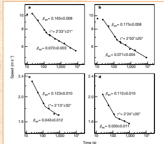
Figure 1 Plots of world record mean speeds against the record time (at November 1999). a,b , Running, and c,d , swimming records: for men ( a,c ), we consider 11 races (200 m, 400 m, 800 m, 1,600 m, 1,500 m, the mile, 3,000 m, 5,000 m, 10,000 m, 1 hour, and marathon); the same races are considered for women ( b,d ), apart from the 1 hour race. Lines represent the best fits. The scaling exponents \beta and characteristic times \tau^* of the breakpoints are shown; characteristic times have been determined by using a \chi^2 minimization on a broken power law. Triangles in a,b represent the 100 m race, which is excluded from the analysis because the mean speed is strongly affected by the standing start of athletes.
