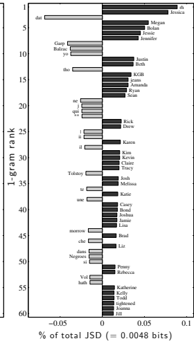
JSD flux contributions: 1970s to 1980s Relative frequency threshold: f_{thr} = 10^{-5}
