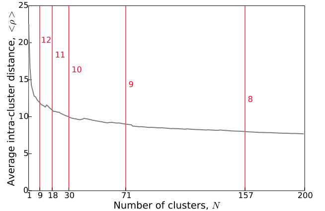
Figure 10. Average intra-cluster distance \langle \rho \rangle as a function of cluster number N . Red lines mark the first occurrence in which the average of the intra cluster distance of the N motif clusters had a value below 12, 11, 10, 9, and 8 (red text beside each line) points respectively. The next cut for 7 points gives 343 motifs.
