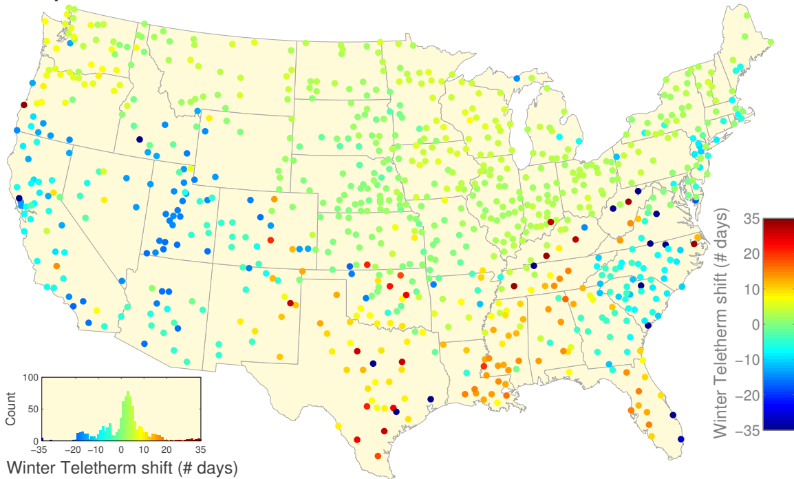
FIG. S11. Teletherm shifts comparing the quarter centuries at the ends of the 1937 to 2012. A: Summer Teletherm shifts comparing the 25 year period 1938–1962 relative to 1912–1937 (837 out of 1218, 68.72%, stations have acceptable data). B: Winter Teletherm shifts comparing 1937/1938–1962/1963 relative to 1912/1913–1936/1937 (838 out of 1218, 68.80%, stations have acceptable data).
