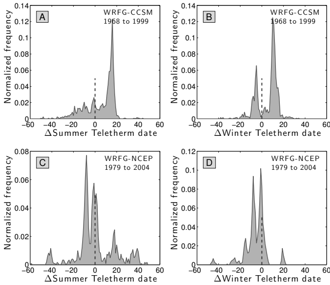
FIG. 7. Distributions of errors in days for the Summer and Winter Teletherms at all stations when comparing measured temperatures to the Community Climate Systems Model (CCSM) (version 3) [16] and the National Centers for Environmental Prediction Climate Forecast System Model (NCEP) [17, 18]. The differences are to be interpreted as how many days the models are “off” from the real data. A positive \Delta means the model’s Teletherm occurs later in the year than the measured one.
