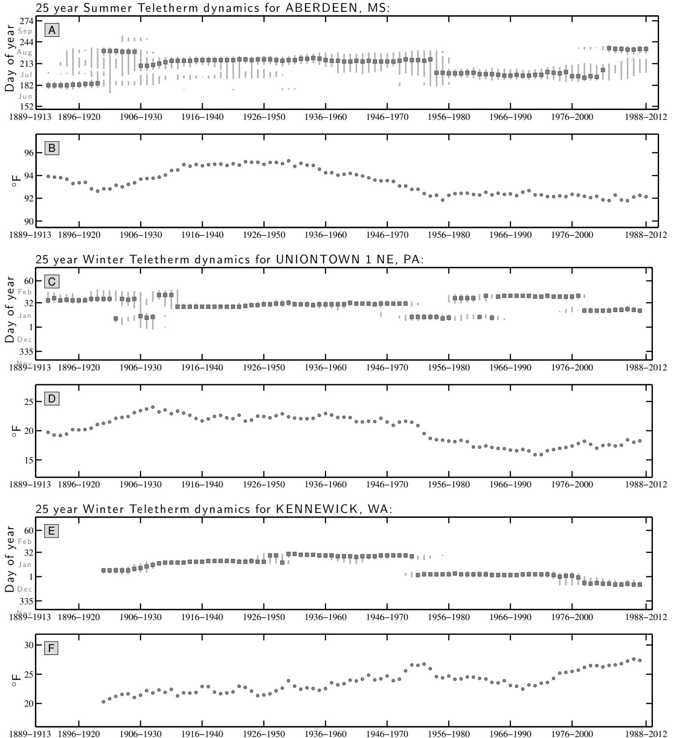
FIG. 4. Dynamics of 25 year Teletherm dates, periods, extents, and temperatures for three example locations displaying abrupt switchings in time and gradual increases and decreases of temperature. We provide sets of these plots for 50, 25, and 10 year Teletherms for all 1218 stations in the Supporting Information (Files S28, S29, and S30). The same plots are also available at http://compstorylab.org/share/papers/dodds2015c/places.html .
