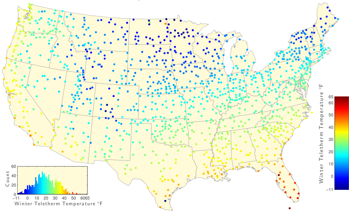
FIG. S2. Winter Teletherm temperatures for the full data set (1853–2012). Teletherm temperatures are determined by smoothing the average daily maximum and minimum temperatures; see main text for details.
