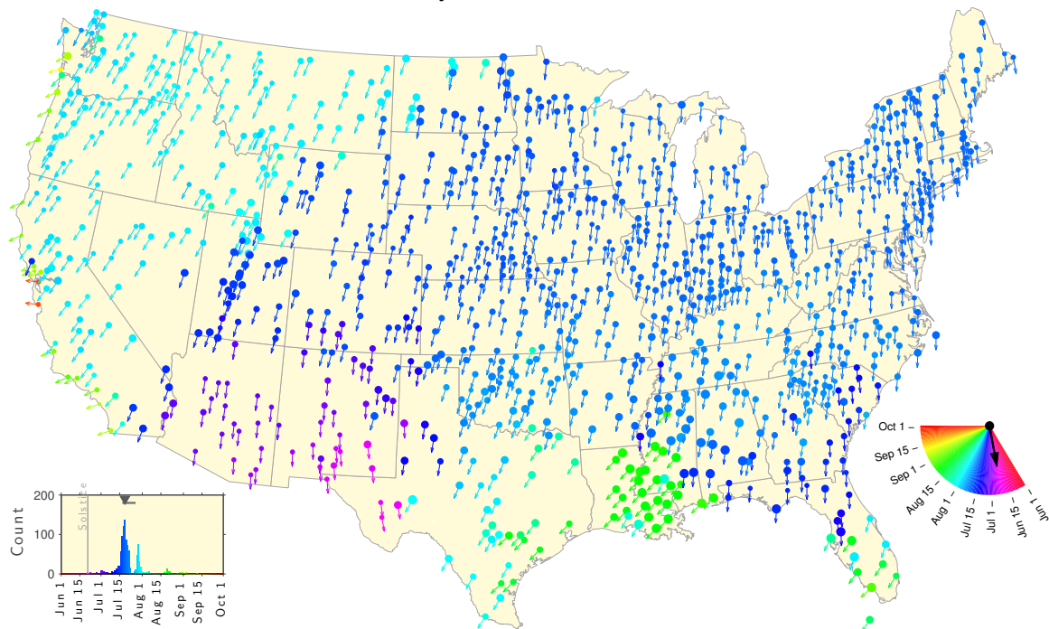
FIG. S5. Map of the Summer Teletherms and Teletherm Extents estimated for the year ranges 1963–2012, to be compared with the preceding map in Fig. S4. Fig. 6A in the main text maps the changes in the Summer Teletherm between these two periods.
