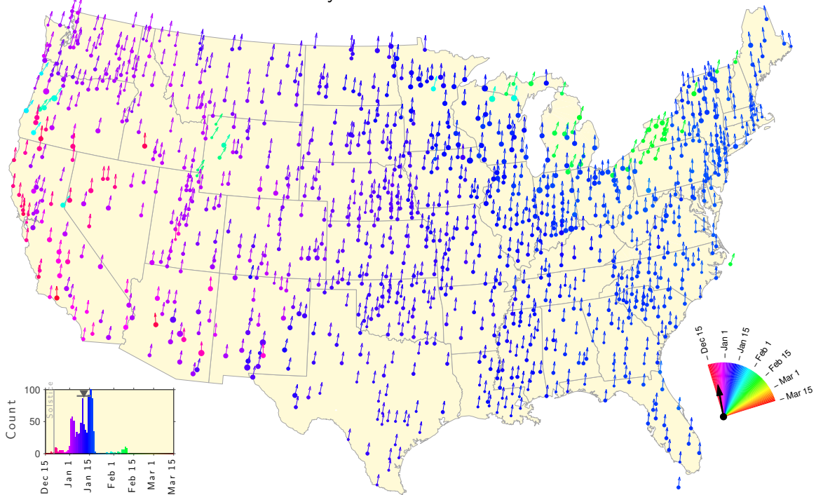
FIG. S7. Map of the Winter Teletherms and Teletherm Extents estimated for the year ranges 1962–2011, to be compared with the preceding map in Fig. S6. See Fig. 6B for a map of the changes.
