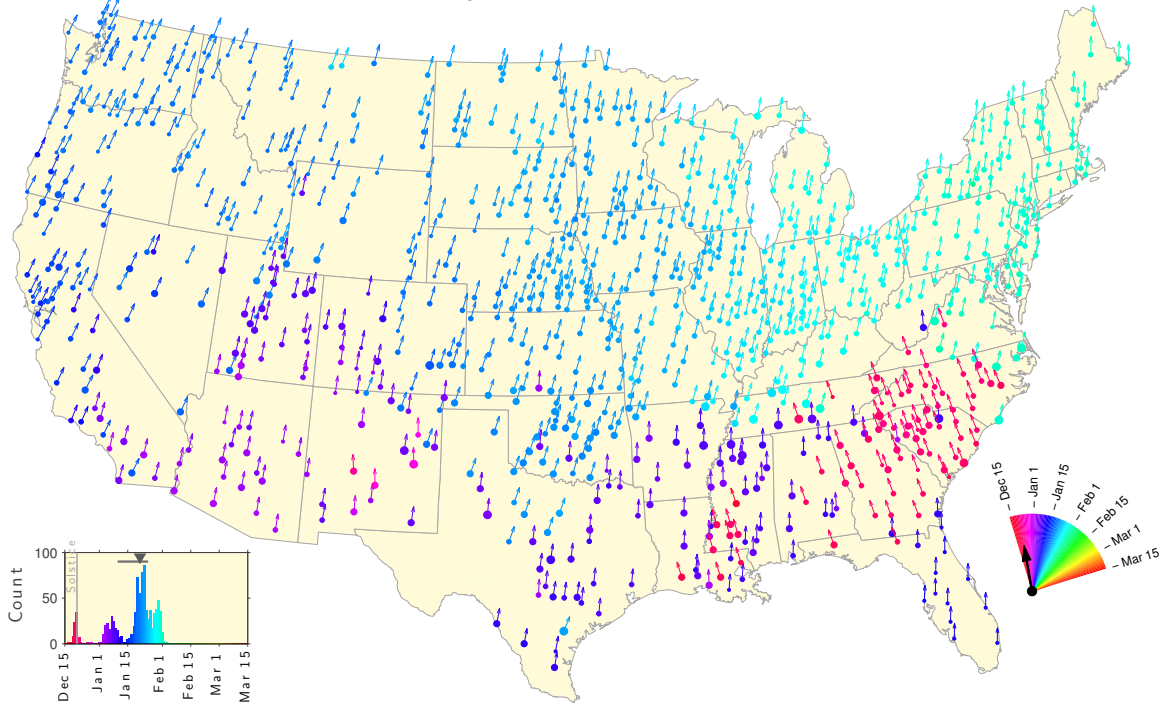
FIG. S6. Map of the Winter Teletherms and Teletherm Extents estimated for the 50 year range 1912–1961, to be compared with the equivalent map for 1962–2011 in Fig. S7. Fig. 6B in the main text maps the changes in Winter Teletherms between these two periods. In the bottom left histogram, the gray horizontal line shows the interquartile range and the inverted triangle the median.
