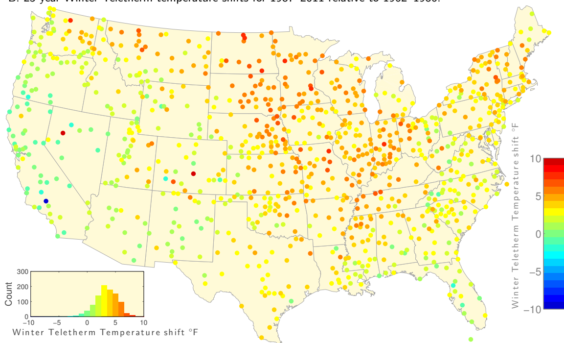
FIG. S17. Teletherm temperature shifts comparing the quarter centuries at the ends of the 1962 to 2012. A: Summer Teletherm temperature shifts comparing the 25 year period 1988–2012 relative to 1963–1987. B: Winter Teletherm temperature shifts comparing 1987/1988–2011/2012 relative to 1962/1963–1986/1987.
