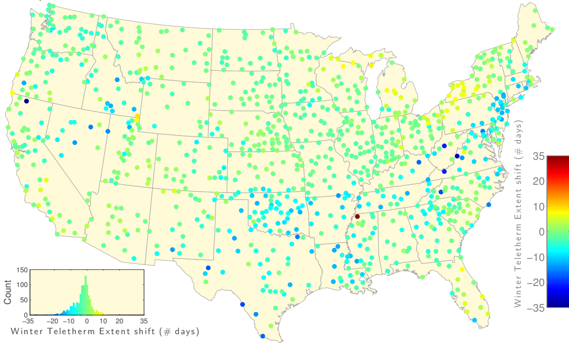
B. 25 year Winter Teletherm extents shifts for 1962–1986 relative to 1937–1961:
