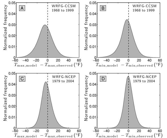
FIG. 8. Comparison between predicted daily maximum and minimum temperatures generated by two climate models (CCSM and NCEP) relative to real measurements for all stations.
