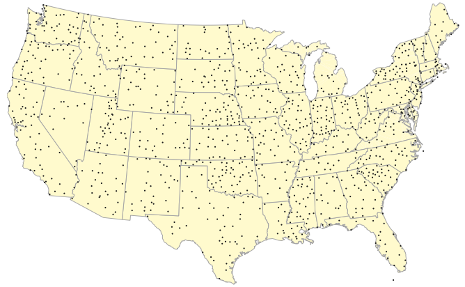
FIG. 1. Locations of 1218 weather stations represented in the United States Historical Climatology Network (USCHN) data set (version 2.5 through 2012) [14]. The distribution indicates relatively uniform coverage of the 48 contiguous states.
