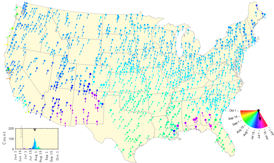
FIG. S4. Map of the Summer Teletherms and Teletherm Extents estimated for the 50 year range 1913–1962, to be compared with the equivalent map for 1963–2012 in Fig. S5. Fig. 6A in the main text maps the changes in Summer Teletherms between these two periods. Relatively few Summer Teletherms have remained stable with the majority shifting to an earlier date. In the bottom left histograms, the gray horizontal line shows the interquartile range and the inverted triangle the median.
