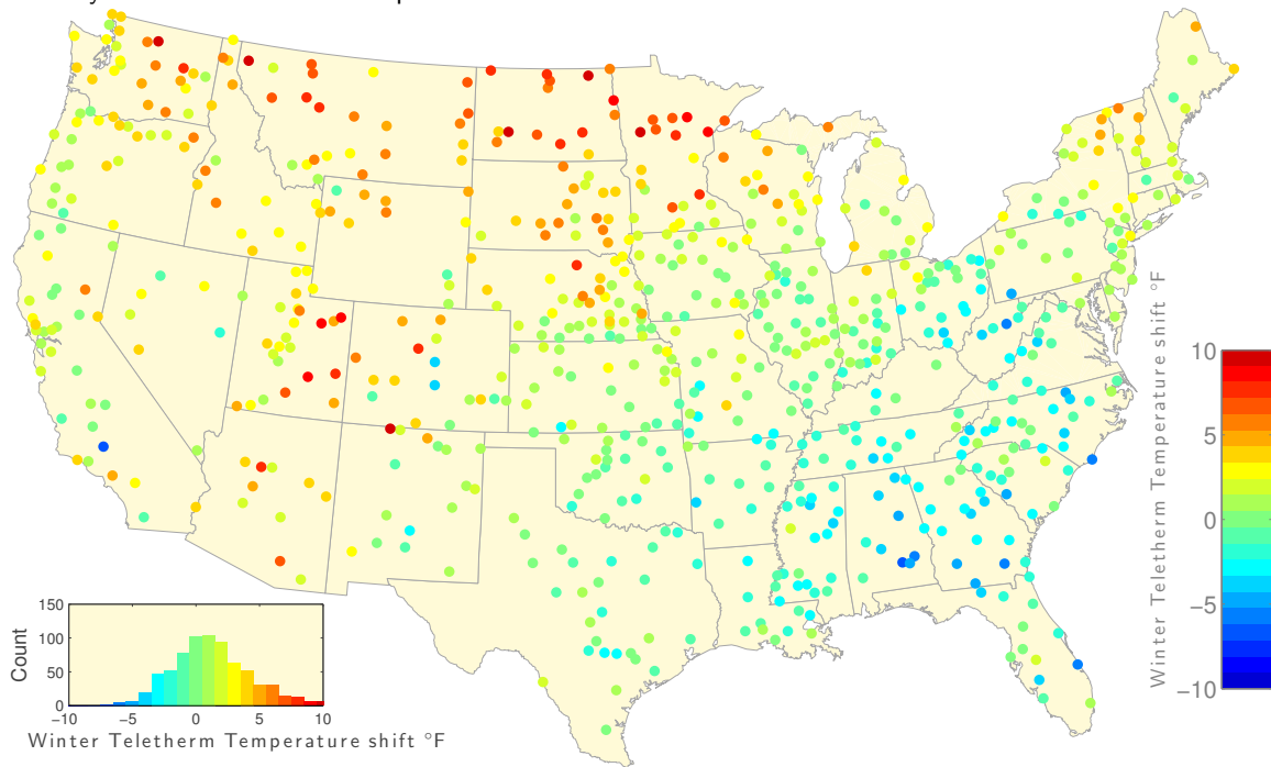
FIG. S14. Teletherm temperature shifts comparing the quarter centuries at the ends of the 1912 to 2012. A: Summer Teletherm temperature shifts comparing the 25 year periods 1988–2012 relative to 1912–1937. B: Winter Teletherm temperature shifts comparing 1987/1988–2011/2012 relative to 1912/1913–1936/1937.
