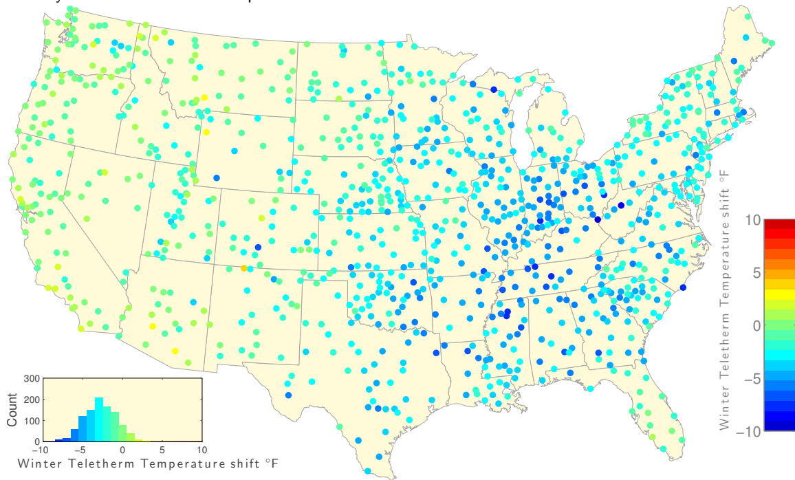
FIG. S16. Teletherm temperature shifts comparing the quarter centuries at the ends of the 1937 to 1987. A: Summer Teletherm temperature shifts comparing the 25 year period 1963–1987 relative to 1938–1962. B: Winter Teletherm temperature shifts comparing 1961/1962–1985/1986 relative to 1937/1938–1961/1962.
