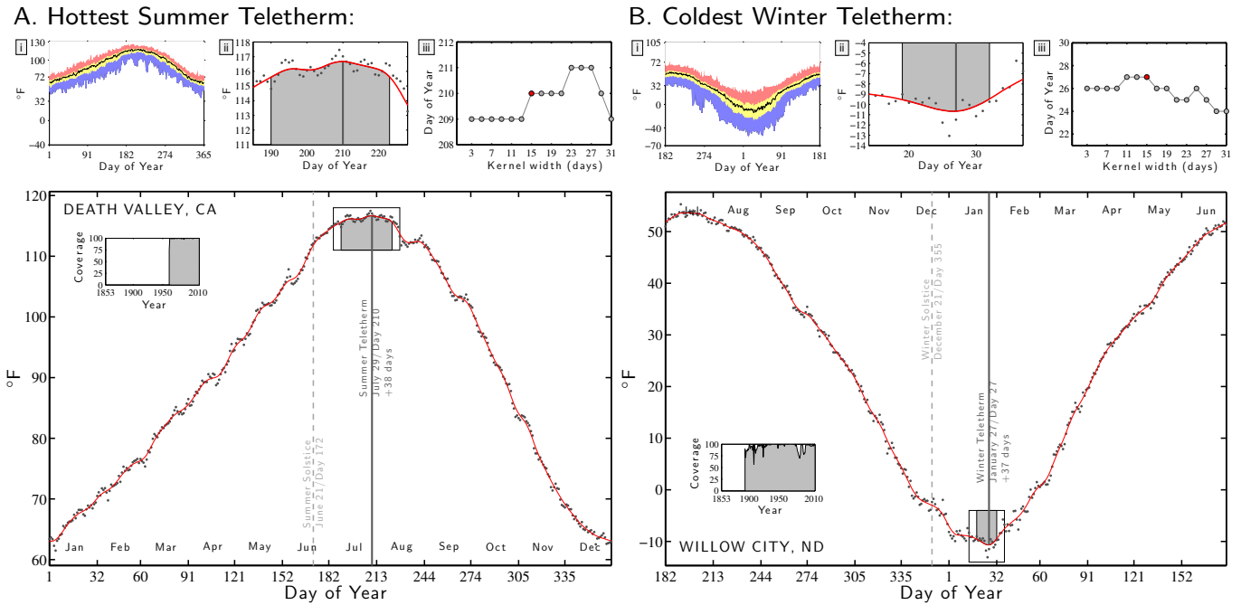
FIG. 2. Plots establishing Teletherm date and Teletherm Periods for the examples of A : the hottest summer Teletherm (Death Valley, California) and B : the coldest winter Teletherm (Willow City, North Dakota). The main plots in A and B show the average daily maximum and minimum temperature (black dots) along with a smoothed curve formed using a Gaussian Kernel (solid red). For all minimum temperature analyses, we wrap the year from July 1 to June 30. The main plots' insets show the fraction of error-free recording for each year. Subplot i : Representation of the spectrum of maximum/minimum temperatures per day of the year. The black curve indicates the median, the blue area indicates lowest to first quartile, yellow the inter-quartile range, and red the fourth quartile. Subplot ii : Expansion of the inset around the Teletherm in the main plot. The dark gray vertical line indicates the Teletherm and the lighter gray region the Teletherm Period which we define as the days for which the smoothed maximum/minimum temperature curve is within 2% of the Teletherm's temperature, relative to the dynamic range of the smoothed curve over the entire 365 days. Subplot iii : Robustness diagnostic showing how the Teletherm date varies as a function of Kernel width. We use 15 days, marked in red. See the main text for further details. See Fig. 3 for four more extreme Teletherm examples. We provide Teletherm plots for the maximum and minimum temperatures for all 1218 stations in the Supporting Information (Files S22 and S23) and in the paper's online appendices at http://compstorylab.org/share/papers/dodds2015c .
