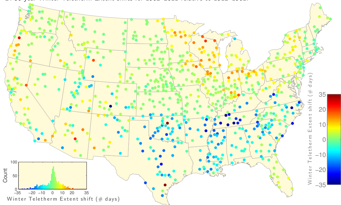
FIG. S9. Shifts for the Winter Teletherm for A : Temperature and B : Extent derived from Figs. S6 and S7.
