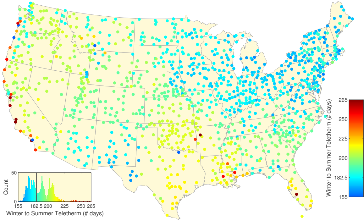
FIG. S3. Number of days from the Winter to the Summer Teletherm. The vertical gray line in the histogram indicates half of a standard 365 day year. The variation is substantial with the northeast showing as short a span as just over 5 months and the west coast as much as 9 months.
