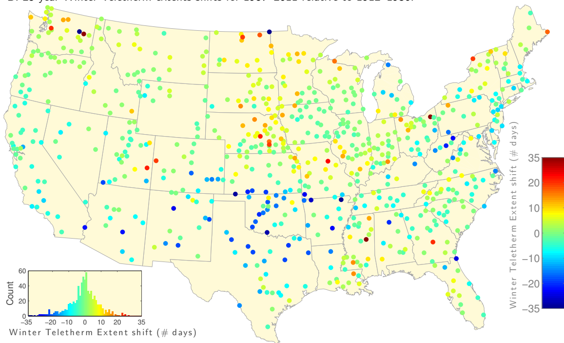
FIG. S18. Teletherm extent shifts comparing the quarter centuries at the ends of the 1912 to 2012. A: Summer Teletherm extent shifts comparing the 25 year periods 1988–2012 relative to 1912–1937. B: Winter Teletherm extent shifts comparing 1987/1988–2011/2012 relative to 1912/1913–1936/1937.
