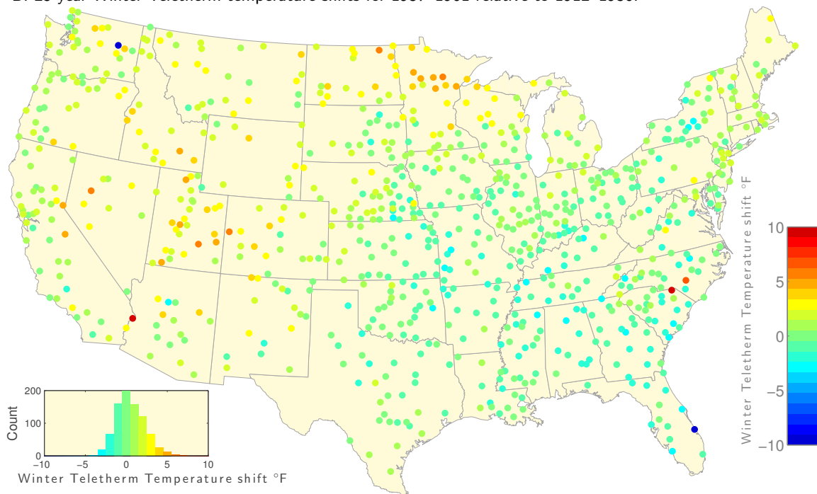
FIG. S15. Teletherm temperature shifts comparing the quarter centuries at the ends of the 1912 to 1963. A: Summer Teletherm temperature shifts comparing the 25 year period 1938–1962 relative to 1912–1937. B: Winter Teletherm temperature shifts comparing 1937/1938–1962/1963 relative to 1912/1913–1936/1937.
