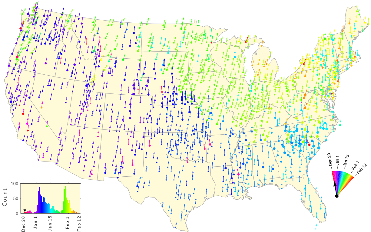
FIG. 5. A: Summer Teletherms and B: Winter Teletherms across the contiguous United States based on all data recorded from 1853 to 2012. Arrows point in the direction of the Teletherm's day of year mapped into angles traveling clockwise with December 31st aligned upwards. The sizes of the markers (discs) represent the duration of a location's Teletherm Period. In the case of multiple Teletherm Periods, sizes correspond to the full extent. Colors map to Teletherm dates as indicated by the partial color wheel in the bottom right corner of each map. The black arrows in the color wheels show the location of the Solstices. The histograms shows the distributions of the Summer and Winter Teletherm, using the same colors.
