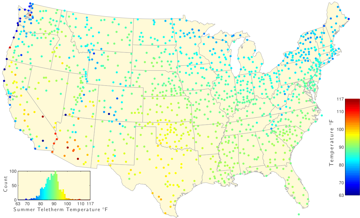
FIG. S1. Summer Teletherm temperatures for the full data set (1853–2012). Teletherm temperatures are determined by smoothing the average daily maximum and minimum temperatures; see main text for details.
