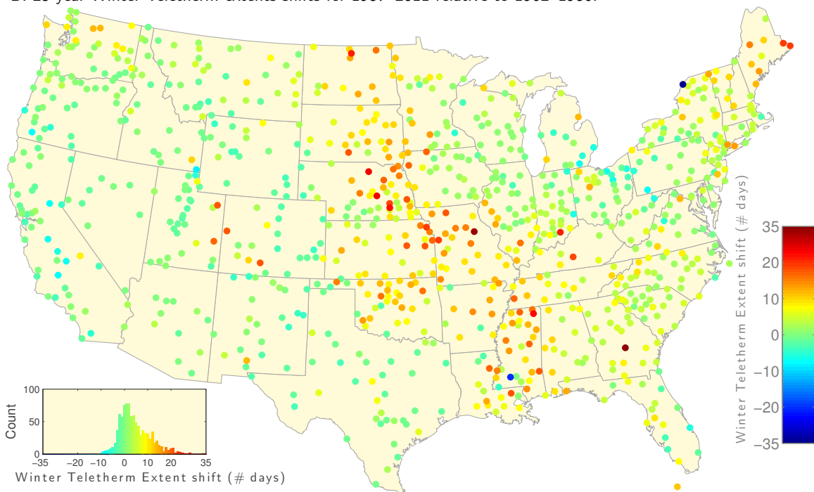
FIG. S21. Teletherm extent shifts comparing the quarter centuries at the ends of the 1962 to 2012. A: Summer Teletherm extent shifts comparing the 25 year period 1988–2012 relative to 1963–1987. B: Winter Teletherm extent shifts comparing 1987/1988–2011/2012 relative to 1962/1963–1986/1987.
