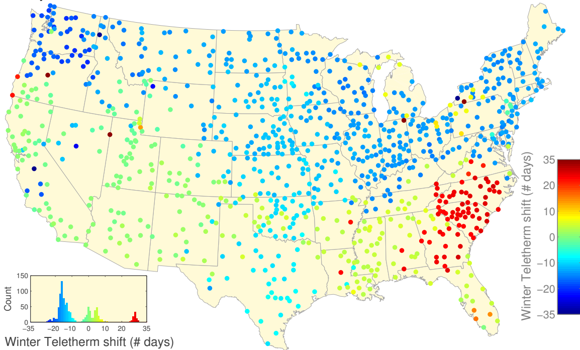
FIG. S12. Teletherm shifts comparing the quarter centuries at the ends of the 1937 to 1987. A: Summer Teletherm shifts comparing the 25 year period 1963–1987 relative to 1938–1962 (1001 out of 1218, 82.18%, stations have acceptable data). B: Winter Teletherm shifts comparing 1961/1962–1985/1986 relative to 1937/1938–1961/1962 (1000 out of 1218, 82.10%, stations have acceptable data).
