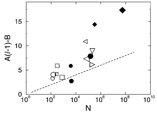
FIG. 13. Comparison between the average path lengths of real scale-free networks and the prediction (63) of scale-free random graphs (dashed line). For each network we have plotted A(\ell-1)-B as a function of N , where A and B are given in the text. The networks included in the figure, indicated by their number in Table I or Table II, are small \circ , I.12; large \circ , I.13; small \square , I.10; medium \square , I.11; large \square , II.13; small \bullet , II.6; medium \bullet , I.2; small \triangleleft , I.6; large \triangleleft , I.8; large \bullet , II.7; \nabla , I.9; \triangleright , I.3; medium \blacklozenge , II.1; large \blacklozenge , II.3.
