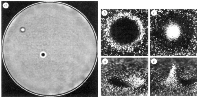
Umbanhowar et al., Nature , 1996 [13]
