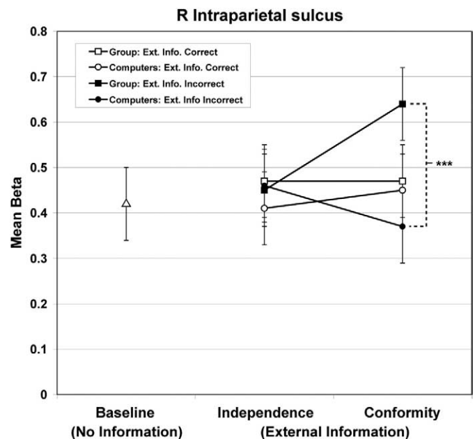
Figure 5. Region-of-interest (ROI) analysis of the right intraparietal sulcus. A 12-mm diameter sphere was centered on the anatomic confluence of effects shown in Figure 4 (Montreal Neurological Institute coordinates: 25, -66, 32). The best-fitting model by Akaike's Information Criterion (Akaike 1974) showed that there was a main effect of source (Group vs. Computers) [ F(1,631) = 6.56 , p = .01 ] and that there was a significant interaction between the source of information and whether the participant gave a correct or incorrect response (i.e., Social Conformity) [ F(1,631) = 5.80 , p = .016 ]. Post hoc comparisons indicated that conforming to incorrect information from the Group was associated with significantly greater activity than conforming to incorrect information from the Computers [***mean difference .271 (SEM .078), F(1,71) = 11.98 , p < .001 ].
