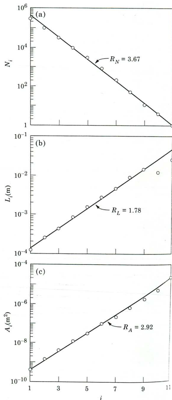
FIG. 17. Morphometric data for the pulmonary arteries of a cat (Fung, 1990, p. 205): (a) branching scaling, number of branches of order i , N_i as a function of order i . The straight-line correlation is from (1) with R_N = 3.67 ; (b) length-order scaling, L_i as a function of i . The straight line correlation is from (2) with R_L = 1.78 ; (c) area-order scaling A_i as a function of i . The straight line correlation is from (20) with R_A = 2.92 .
