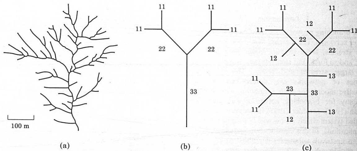
FIG. 1. (a) Example of an actual fourth-order river network; (b) deterministic third-order, binary fractal tree. The third-order stem bifurcates into two second-order branches, the second-order branches bifurcate into two first-order branches; (c) side branches have been added to the binary tree in (b). The third-order branch has two first-order side branches and one second-order side branch. Each second-order branch has a first-order side branch. The Tokunaga ordering system is given.
