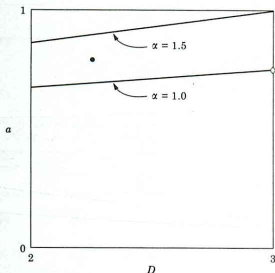
FIG. 16. Dependence of the allometric exponent a on the fractal dimension D for area preserving scaling ( \alpha = 1 ) and A^{3/2} scaling ( \alpha = 3/2 ) from (47). ( \diamond ) is the result given by West et al. (1997) and ( \bullet ) is from the data for the pulmonary arteries of a cat as illustrated in Fig. 17.
