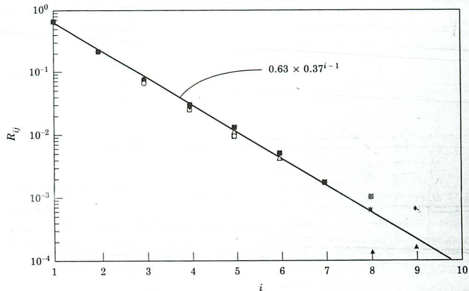
FIG. 11. Dependence of the terms of the ramification matrix R_{ij} for the branching statistics of a diffusion limited aggregation (DLA) cluster on the branch order i for various branch orders j ( j : (+) 1; (*) 2; (x) 3; (○) 4; (□) 5; (◇) 6; (△) 7; (■) 8; (◆) 9; (▲) 10). Branches of order i join branches of order j so that i < j . The data points are for an average of 47 off-lattice DLA clusters each with 10^6 particles (Ossadnik, 1992). The straight-line correlation is with the Tokunaga relation (17) taking c = 2.7 .
