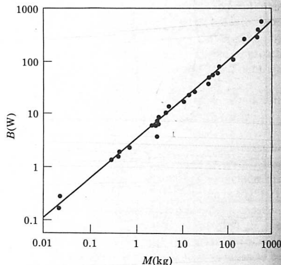
FIG. 15. The dependence of the metabolic rate B on body mass M for a variety of species from mice to elephants (Calder, 1984). The straight-line correlation is from the allometric relation (19) with a a = 0.75 .
