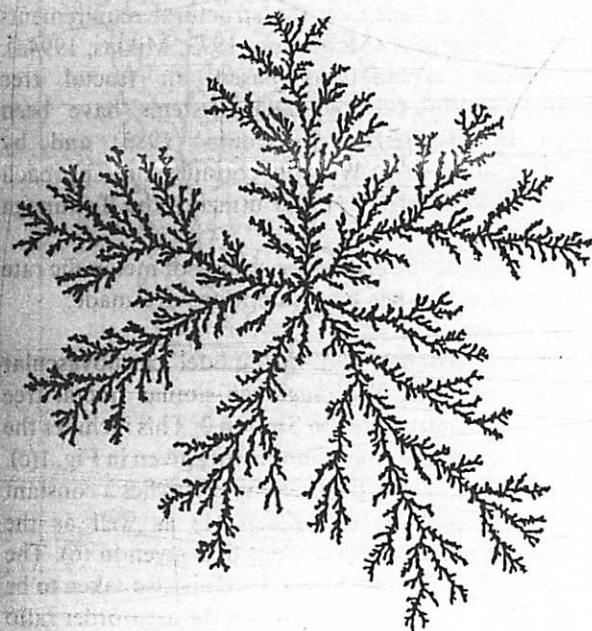
FIG. 10. A two-dimensional, off-lattice DLA cluster with 10^6 particles (Ossadnik, 1992).
