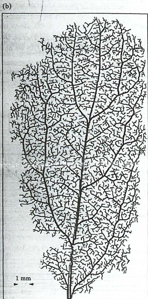
FIG. 12. (a) River network of the Kentucky River basin, Kentucky; (b) vein structure of a side lobe of a mature leaf in Sorbus hybrida (Rosaceae) obtained using a scanning routine on a grey scale image given by Merrill (1978).
