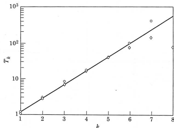
FIG. 14. Dependence of the mean branching ratios T_k on k for the Kentucky River basin illustrated in Fig. 12(a) (○) and for the side lobe of the leaf illustrated in Fig. 12(b) (◇). The straight line correlation is with the Tokunaga relation (6) taking a = 1.2 and c = 2.5 .
