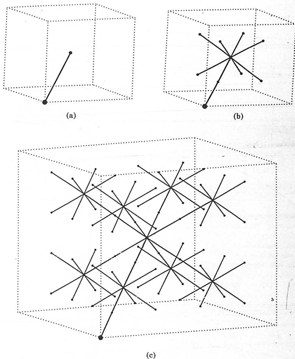
FIG. 8. Deterministic volume filling fractal tree with side branching and R_L = 2 . The construction is based on a body-centered cubic lattice. Tip nodes emit seven branches at each order and internal nodes emit six branches. (a) First-order example; (b) second-order example; (c) third-order example.
