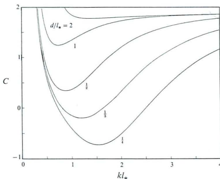
FIGURE 1. The scaling parameter C (3.13) for d/l_* = \frac{1}{4}, \frac{1}{3}, \frac{1}{2}, 1 and 2 . The steep rise of C on the left announces internal resonance between the primary wave and its second harmonic (Wilton's ripples). The asymptotic ( kl_* \uparrow \infty ) value of C is (33 - 2\sqrt{2})/16 = 1.89 .
