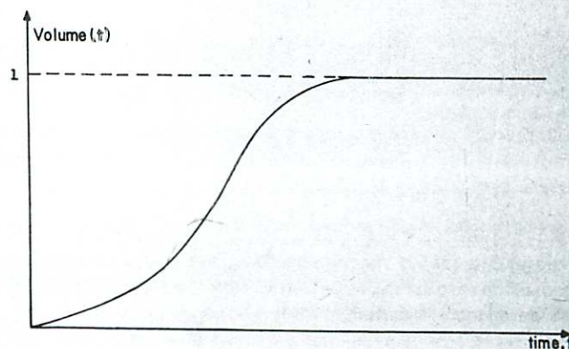
Fig. 2. Effective rainfall volume collected at the trapping state as function of time, resulting from a unit input of precipitation.
