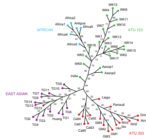
Figure 2. Majority-rule consensus of the most parsimonious trees returned by the cladistic analysis of the tales. Major groups are indicated by regions of PCA (continental type) and indicated by the colored circles. Sub-groups are indicated in the web labels (e.g., "Africa1" refers to "Africa1 = Story of Grandmother Cat" in Cameroon, etc.). The "Indo" and "Indo" labels refer to "Indo-European" variants by particular authors, or their corresponding groups that are discussed in the text have been individual labels. Numbers beside the edges represent the level of support for individual clades assumed by the bootstrap analysis. doi:10.1371/journal.pone.0218111.g002
